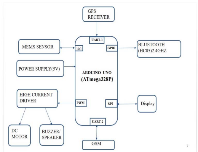
Fig 1: The implemented system block level diagram
